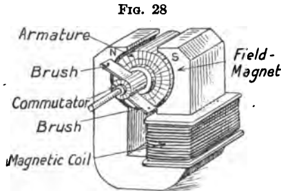
Plan of dynamo.
